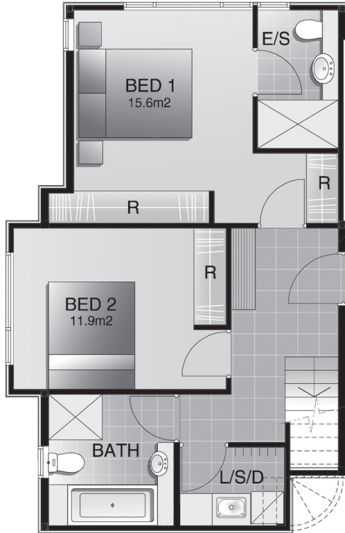
Lower floor of apartment (level 5)
